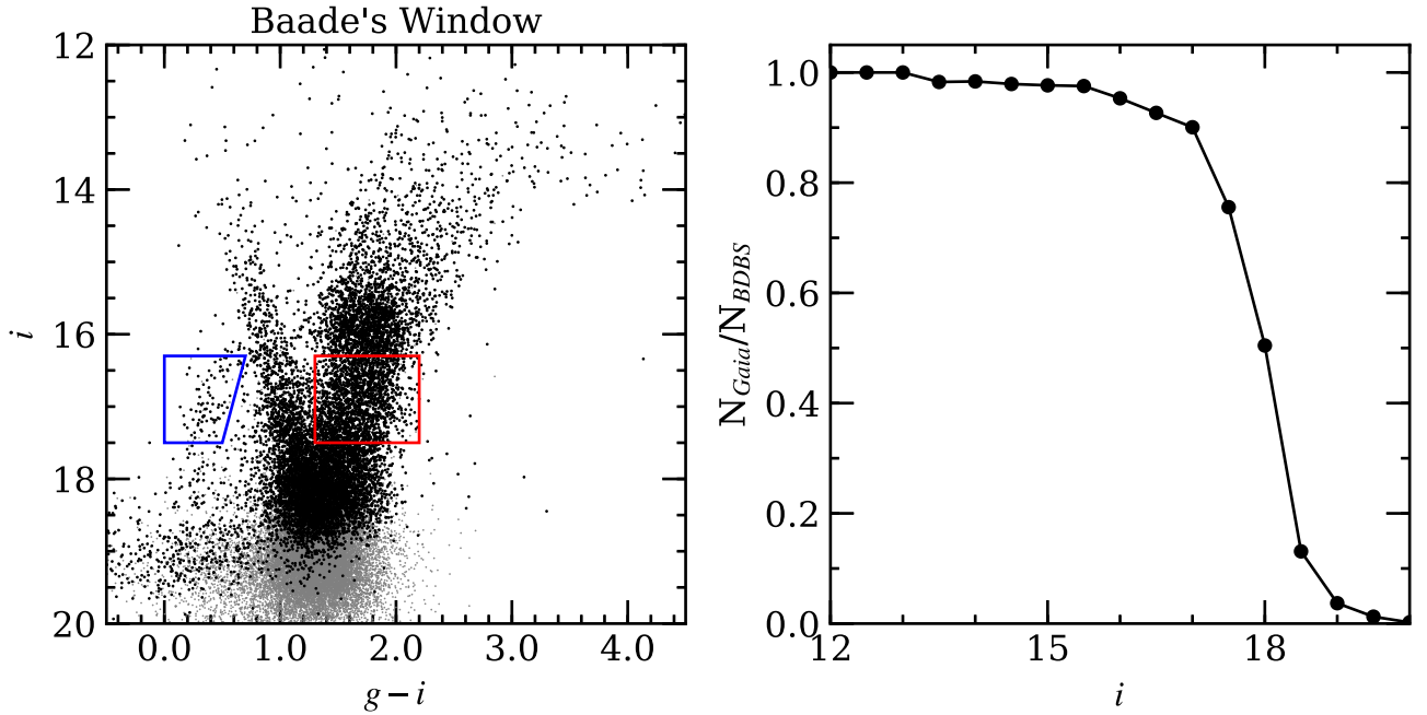
Figure 4. (Left): A colour-magnitude diagram of Baade’s Window ( l, b = (0.9^\circ, -3.9^\circ) ) in the Galactic bulge with selection boxes indicating blue HB and RGB stars. (Right): The fraction of stars with Gaia DR2 matching, as a function of i magnitude. The completeness limit for Gaia DR2 matching is substantially fainter than the red clump, in this field.
