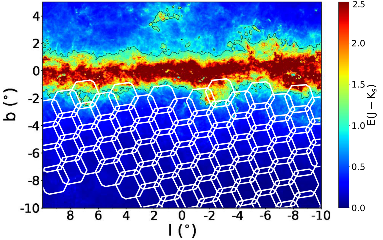
Figure 3. The BDBS fields are superimposed on the reddening map constructed from 1 \times 1 arcmin cells (Simion et al. 2017). At this point, the reddening map is based on data from the VVV survey; we ultimately plan to deredden over the full BDBS footprint.
