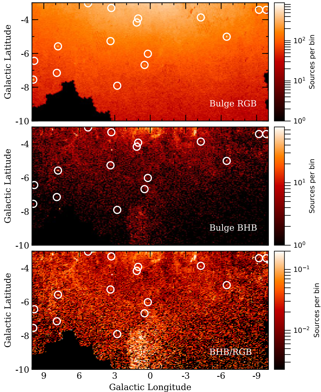
Figure 11. Mapping the blue HB of the Milky Way. Upper panel is the density of RGB stars; center panel is the density of BHB stars as in Fig. 10; the bottom panel is the ratio of BHB/RGB stars.
