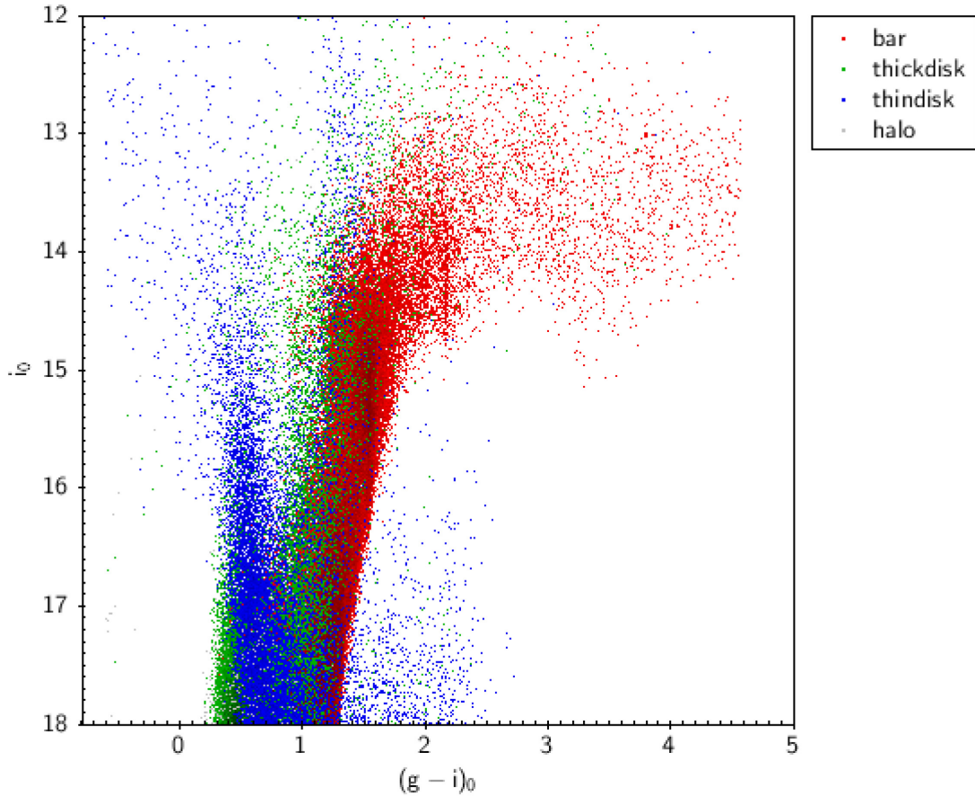
Figure 7. A model CMD of the population towards Baade’s Window ( l, b = (-0.2^\circ, +3.9^\circ) ) covering 0.1 \text{ deg}^2 (see text and the Besancon Galaxy Model; Lagarde et al. 2017). This model breaks down the the CMD by stellar populations as indicated in the legend. Notice that the bright blue population near the red giant branch is dominated by stars in the thin disc, not the bulge.
