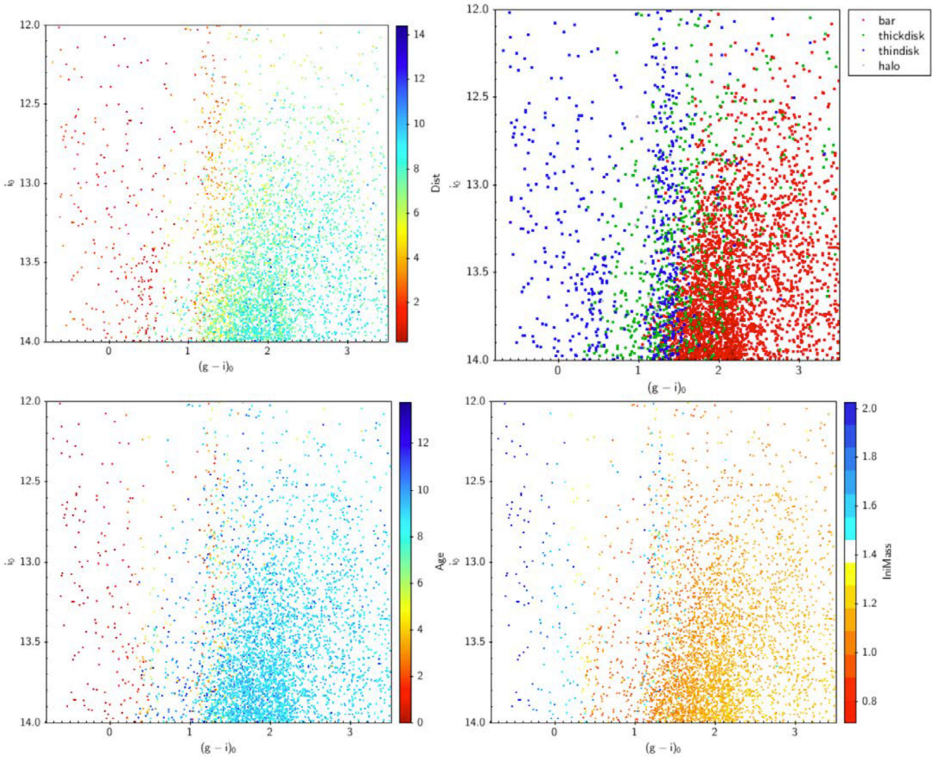
Figure 8. A model CMD of the population towards Baade’s Window ( l, b = (-0.2^\circ, +3.9^\circ) ) covering 0.1 \text{ deg}^2 (see text and the Besancon Galaxy Model; Lagarde et al. 2017). Clockwise from the top are panels showing the distance in kpc, the population (indicated in the legend), the stellar mass, and the age in Gyr. The population proposed by Saha et al. (2019) as the massive blue loop stars would be the blue (disc stars) in the population panel, near i = 12.5 and g - i = 1 . This model would assign the blue plume’ to the foreground disc population, which might plausibly explain the unusual bright extension seen in the red clump near (l, b) = (+8^\circ, -4^\circ) that is seen in Fig. 5.
